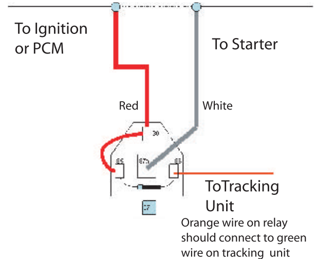
figure 2 - relay wiring diagram
